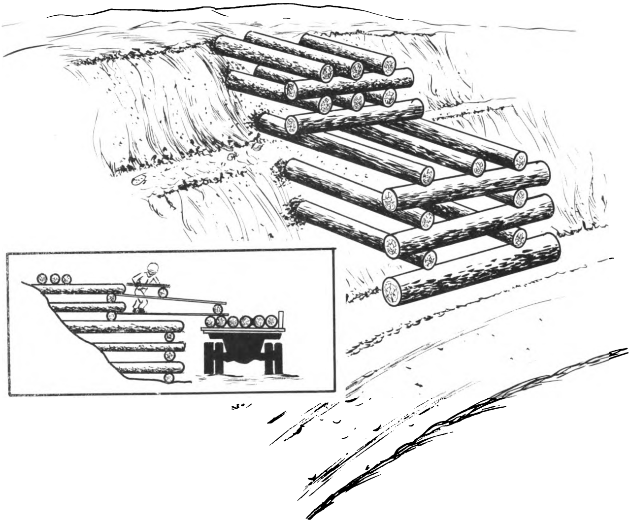
Figure 7-16. Double-deck skidway.
